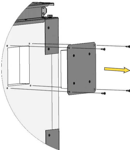
Inspection hole detail
