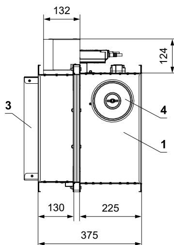
FDMA with spring return actuator
