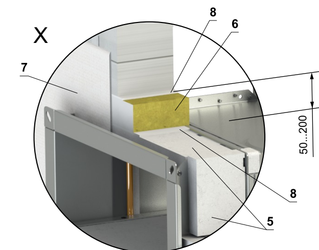
Isolation cover of actuator
