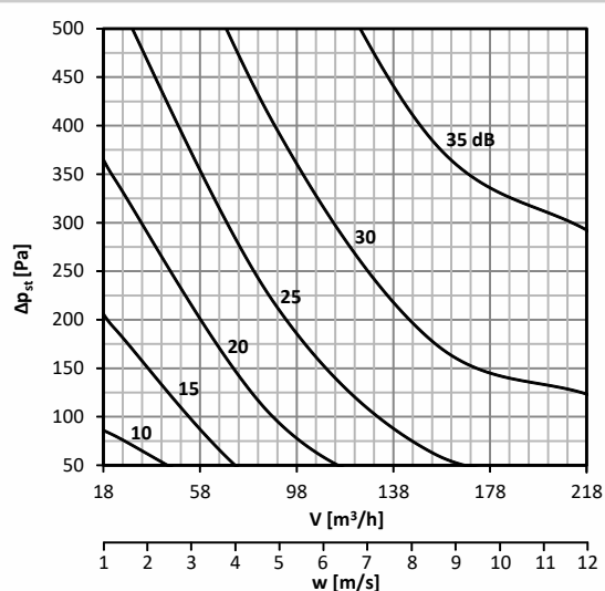
Diagram No. 33 Sound power level L_{WA} [dB(A)] radiated outside the pipeline DN125, with insulation
