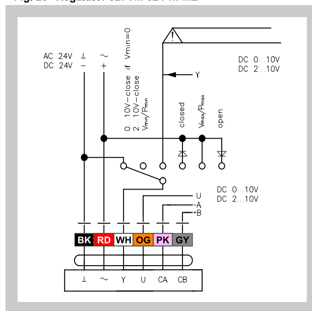
Fig. 20 Regulator 327VM-024-...-MB
