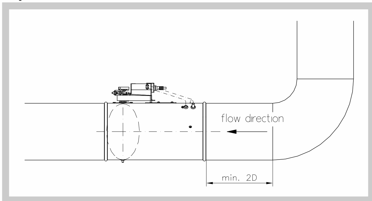
Fig. 33 Recommended distance from bend
