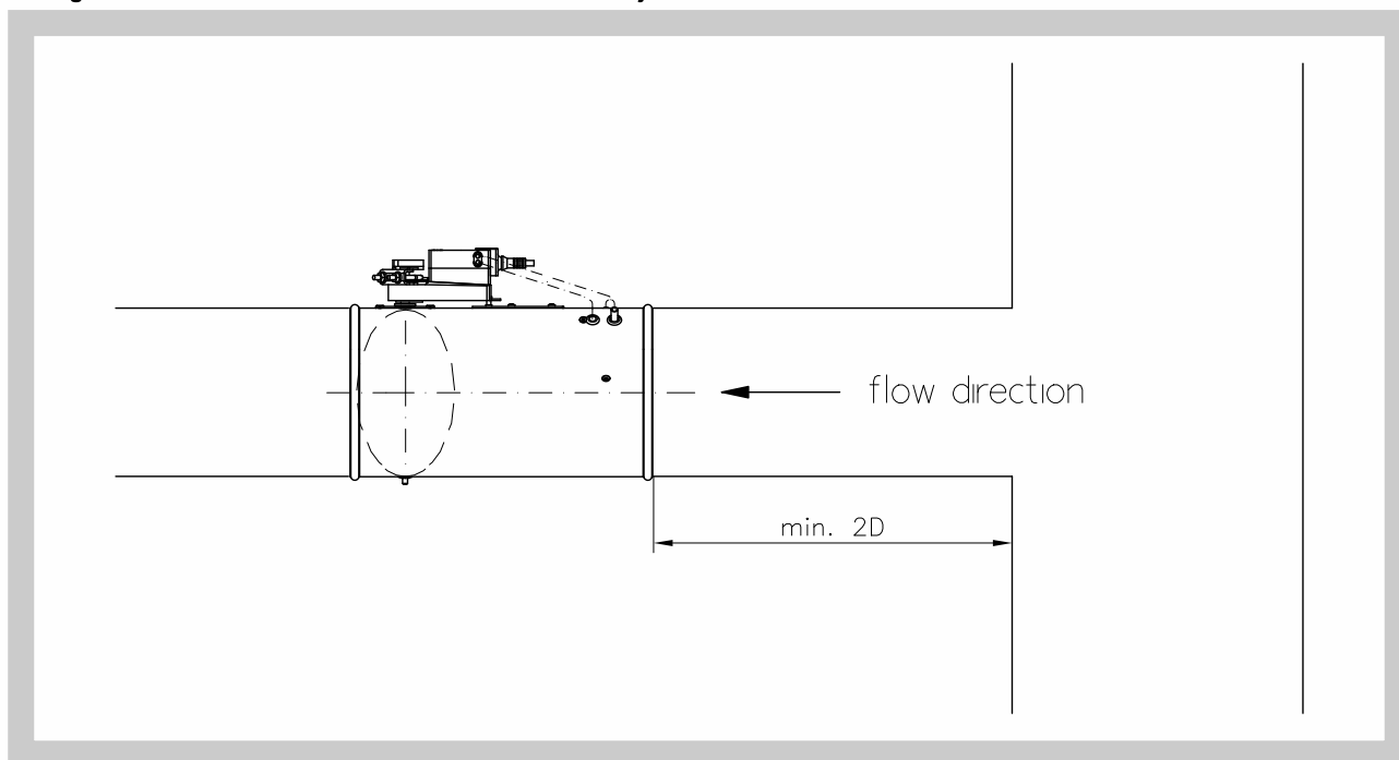
Fig. 32 Recommended distance from double branch joint
