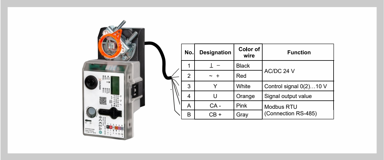
Fig. 18 Regulators 327VM-024-... -MB
