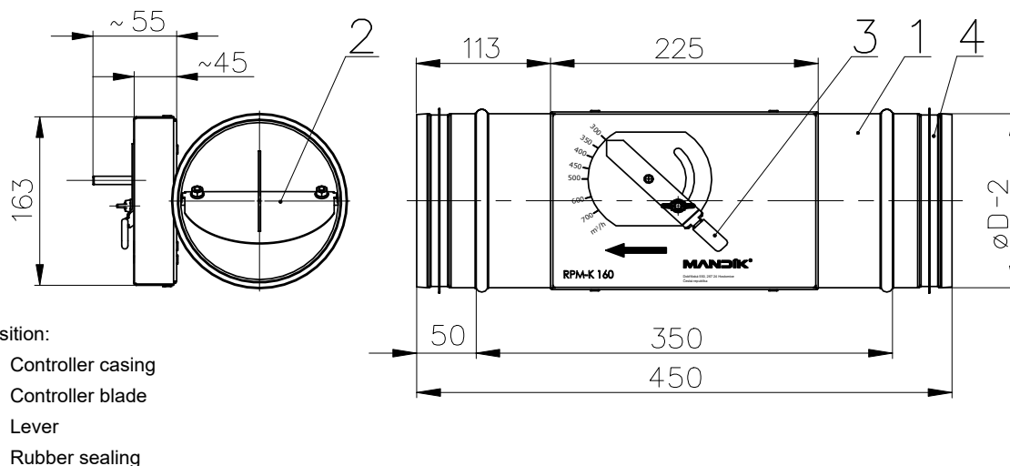
Fig. 3 Constant air volume regulator - with flanges
