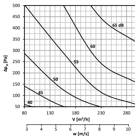
Diagram No. 4 Sound power level L_{WA} [dB(A)] inside the pipeline DN160
