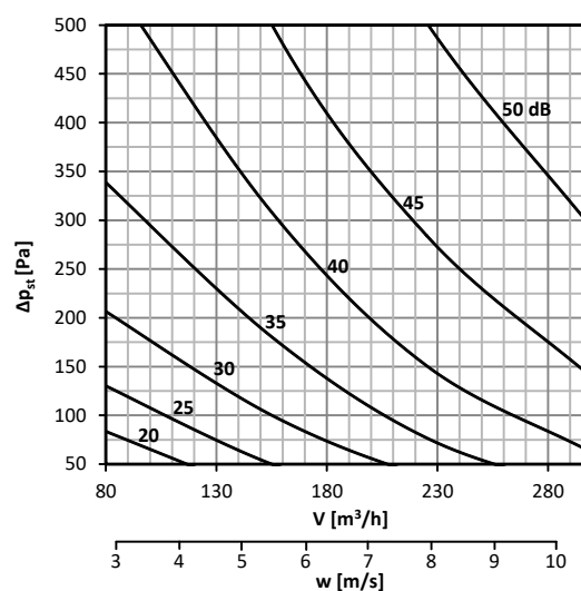
Diagram No. 10 Sound power level L WA [dB(A)] radiated outside the pipeline DN100, without insulation
