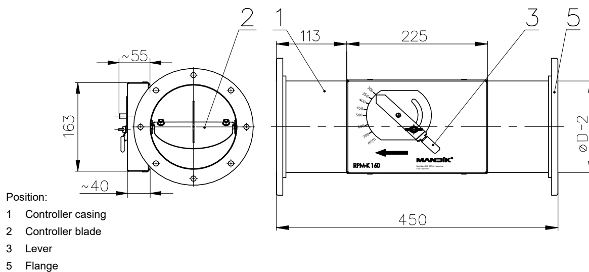
Fig. 4 Constant air volume regulator - with actuating mechanism
