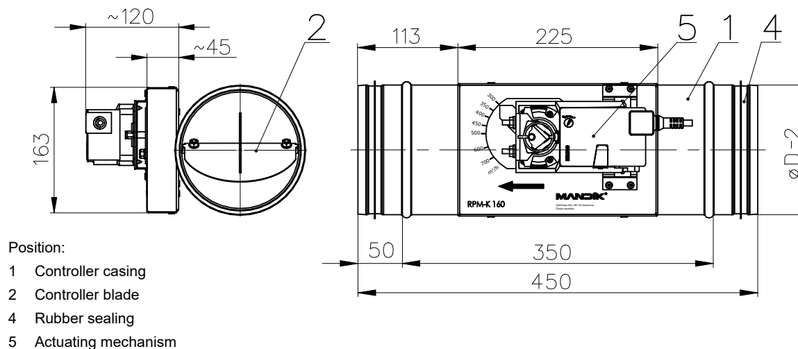
Fig. 4 Constant air volume regulator - with actuating mechanism
