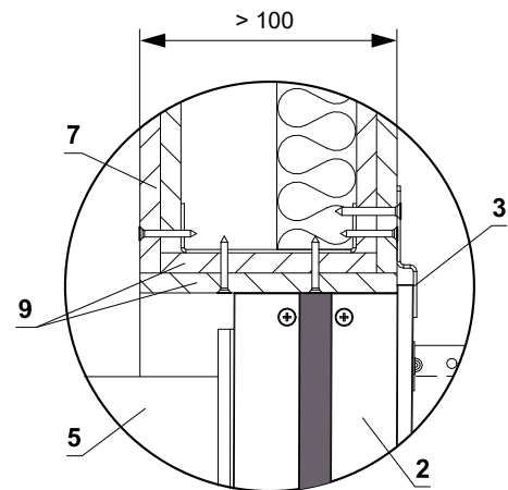
Detail of the wall &gt; 100 mm
