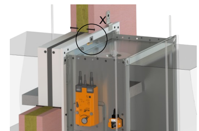
Detail of the wall &gt; 100 mm
