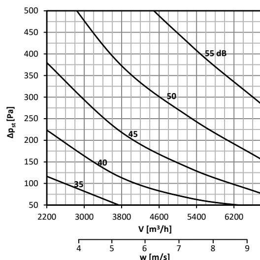
Diagram No. 64 Sound power level L_{WA} [dB(A)] radiated outside the pipeline 600x200, with insulation
