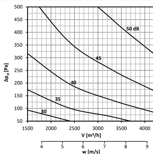
Diagram No. 62 Sound power level L_{WA} [dB(A)] radiated outside the pipeline 500x400, with insulation
