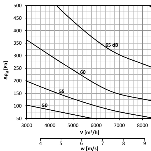
Diagram No. 40 Sound power level L_{WA} [dB(A)] radiated outside the pipeline 500x500, without insulation
