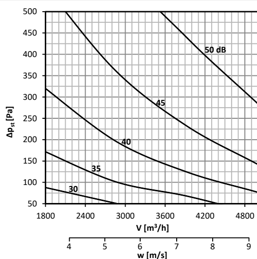
Diagram No. 67 Sound power level L_{WA} [dB(A)] radiated outside the pipeline 600x400, with insulation
