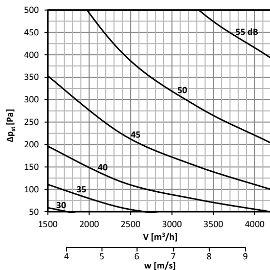
Diagram No. 57 Sound power level L_{WA} [dB(A)] radiated outside the pipeline 400x300, with insulation
