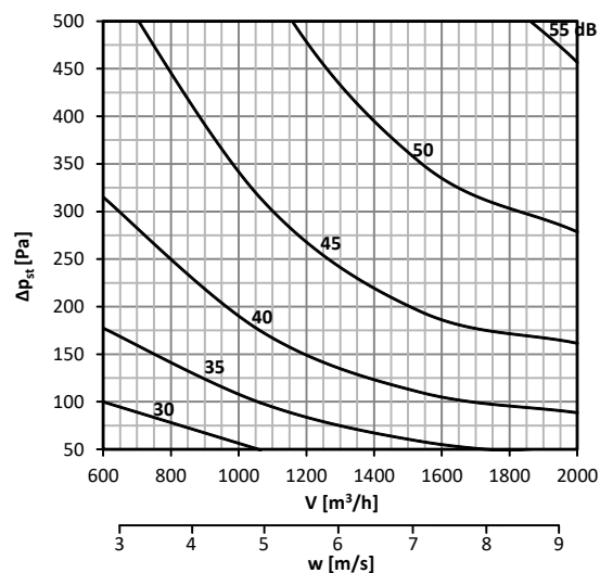
Diagram No. 52 Sound power level L_{WA} [dB(A)] radiated outside the pipeline 300x200, with insulation
