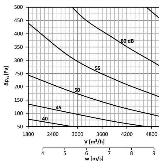
Diagram No. 44 Sound power level L_{WA} [dB(A)] radiated outside the pipeline 600x400, without insulation
