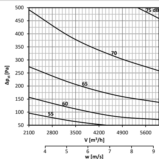
Diagram No. 22 Sound power level L_{WA} [dB(A)] inside the pipeline 600x500
