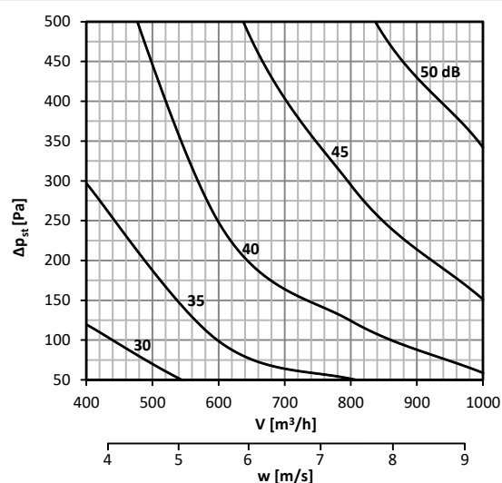
Diagram No. 50 Sound power level L_{WA} [dB(A)] radiated outside the pipeline 300x100, with insulation
