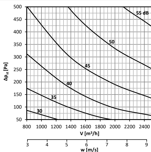
Diagram No. 55 Sound power level L_{WA} [dB(A)] radiated outside the pipeline 400x200, with insulation
