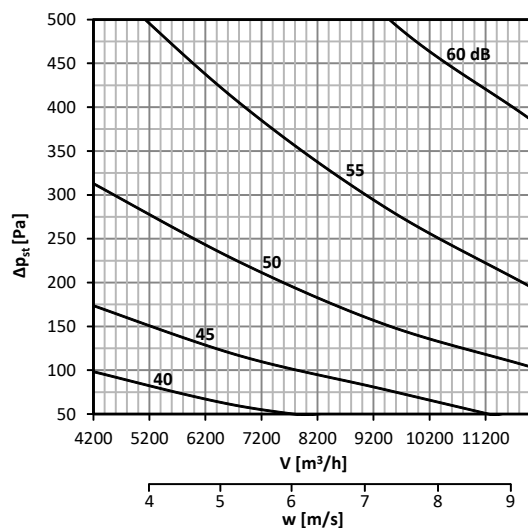
Diagram No. 69 Sound power level L_{WA} [dB(A)] radiated outside the pipeline 600x600, with insulation
