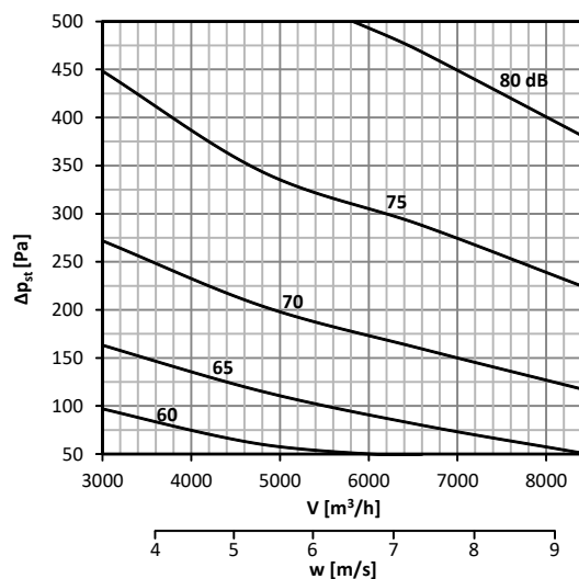
Diagram No. 17 Sound power level L_{WA} [dB(A)] inside the pipeline 500x500
