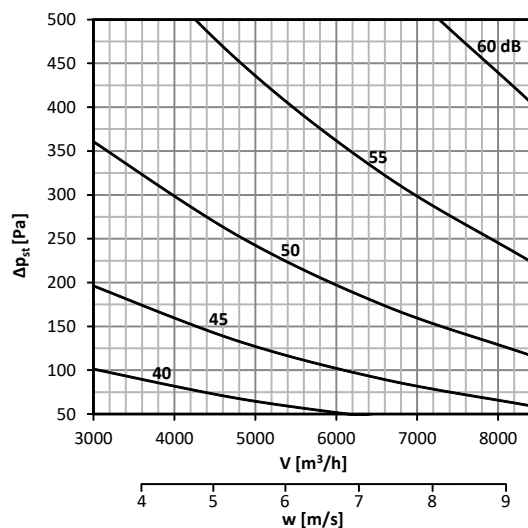
Diagram No. 63 Sound power level L_{WA} [dB(A)] radiated outside the pipeline 500x500, with insulation
