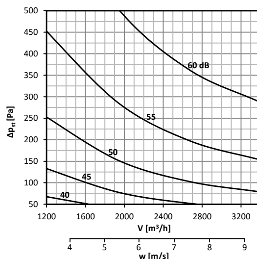
Diagram No. 35 Sound power level L_{WA} [dB(A)] radiated outside the pipeline 400x400, without insulation
