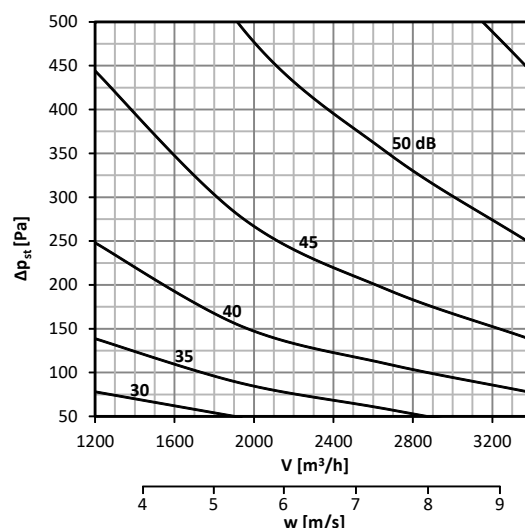
Diagram No. 58 Sound power level L_{WA} [dB(A)] radiated outside the pipeline 400x400, with insulation
