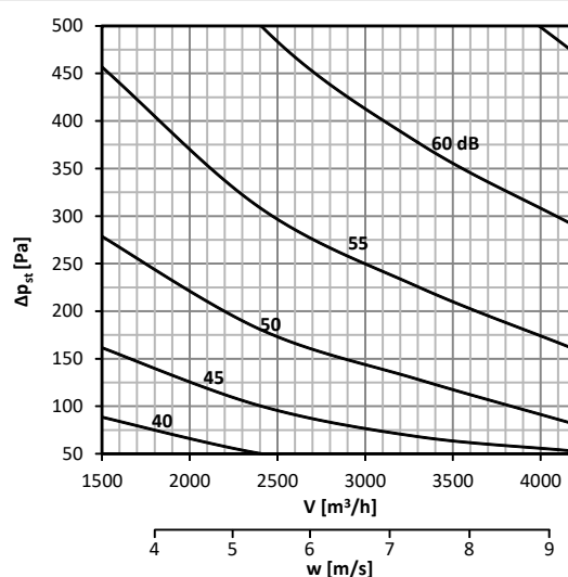
Diagram No. 39 Sound power level L_{WA} [dB(A)] radiated outside the pipeline 500x400, without insulation
