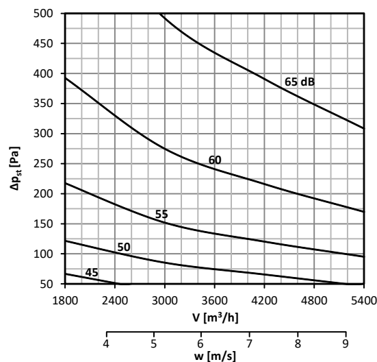
Diagram No. 35 Sound power level L_{WA} [dB(A)] radiated outside the pipeline 400x400, without insulation
