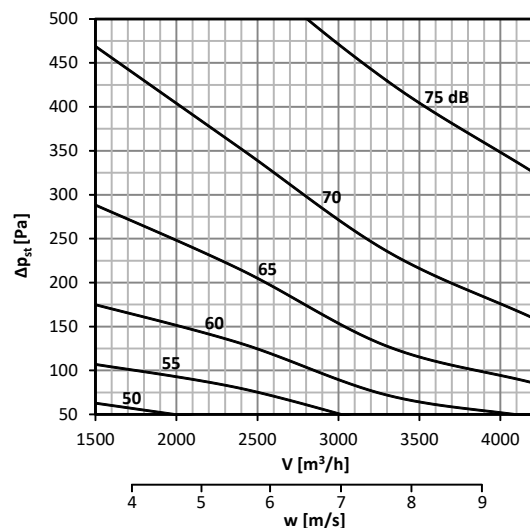
Diagram No. 11 Sound power level L_{WA} [dB(A)] inside the pipeline 400x300
