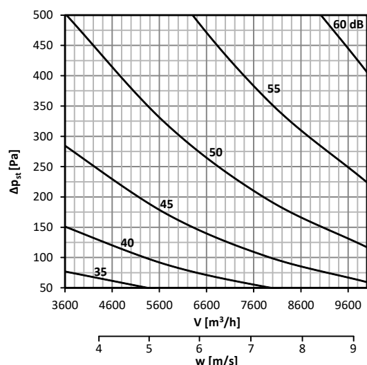
Diagram No. 68 Sound power level L_{WA} [dB(A)] radiated outside the pipeline 600x500, with insulation
