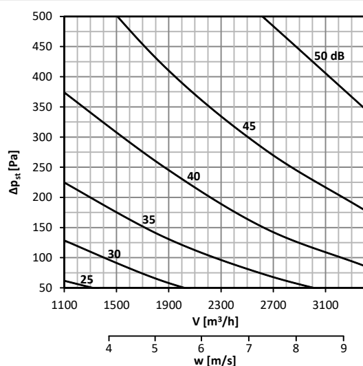
Diagram No. 61 Sound power level L_{WA} [dB(A)] radiated outside the pipeline 500x300, with insulation
