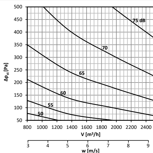
Diagram No. 9 Sound power level L_{WA} [dB(A)] inside the pipeline 400x200
