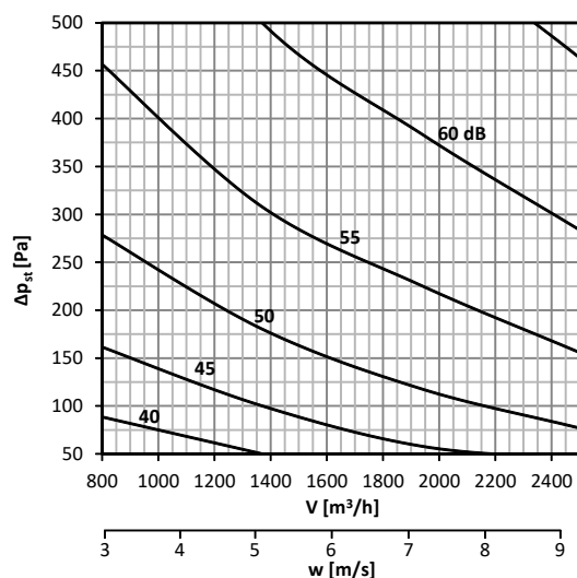
Diagram No. 32 Sound power level L_{WA} [dB(A)] radiated outside the pipeline 400x200, without insulation
