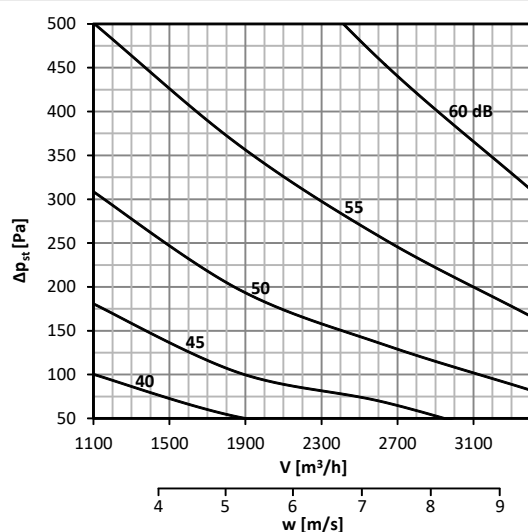
Diagram No. 38 Sound power level L_{WA} [dB(A)] radiated outside the pipeline 500x300, without insulation
