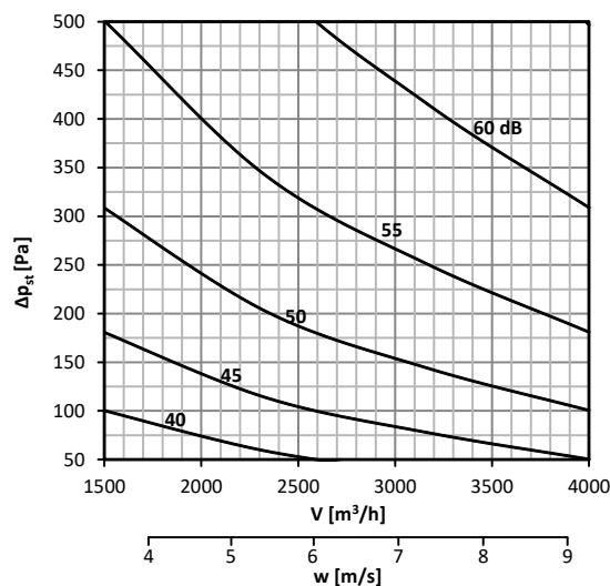
Diagram No. 41 Sound power level L_{WA} [dB(A)] radiated outside the pipeline 600x200, without insulation
