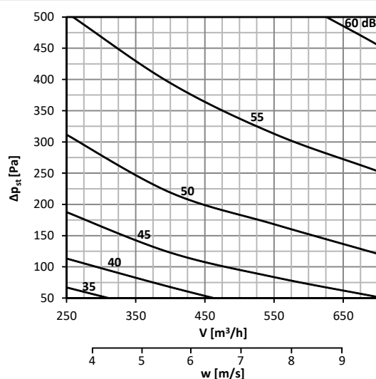
Diagram No. 26 Sound power level L_{WA} [dB(A)] radiated outside the pipeline 200x200, without insulation
