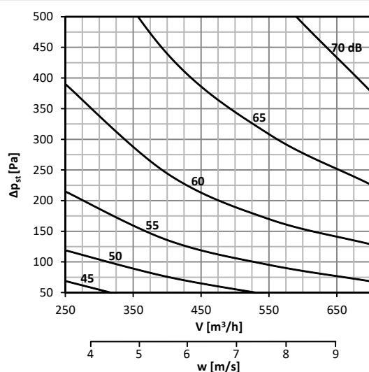
Diagram No. 3 Sound power level L_{WA} [dB(A)] inside the pipeline 200x200
