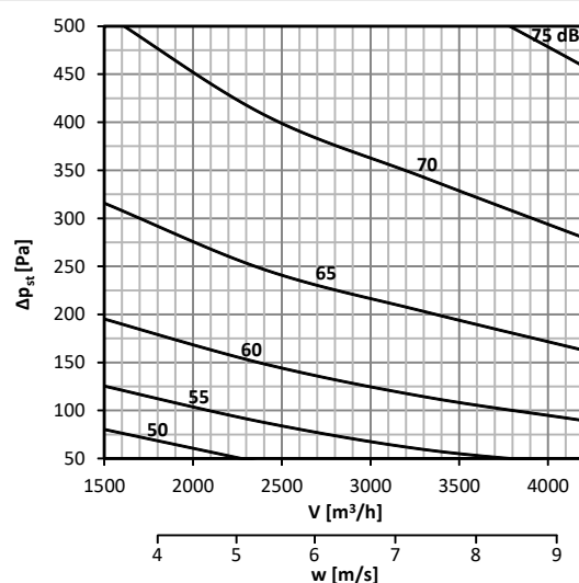
Diagram No. 16 Sound power level L_{WA} [dB(A)] inside the pipeline 500x400
