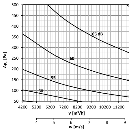
Diagram No. 46 Sound power level L_{WA} [dB(A)] radiated outside the pipeline 600x600, without insulation
