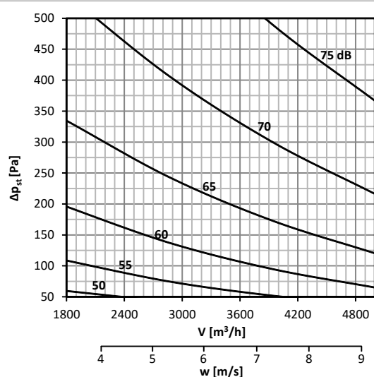
Diagram No. 21 Sound power level L_{WA} [dB(A)] inside the pipeline 600x400
