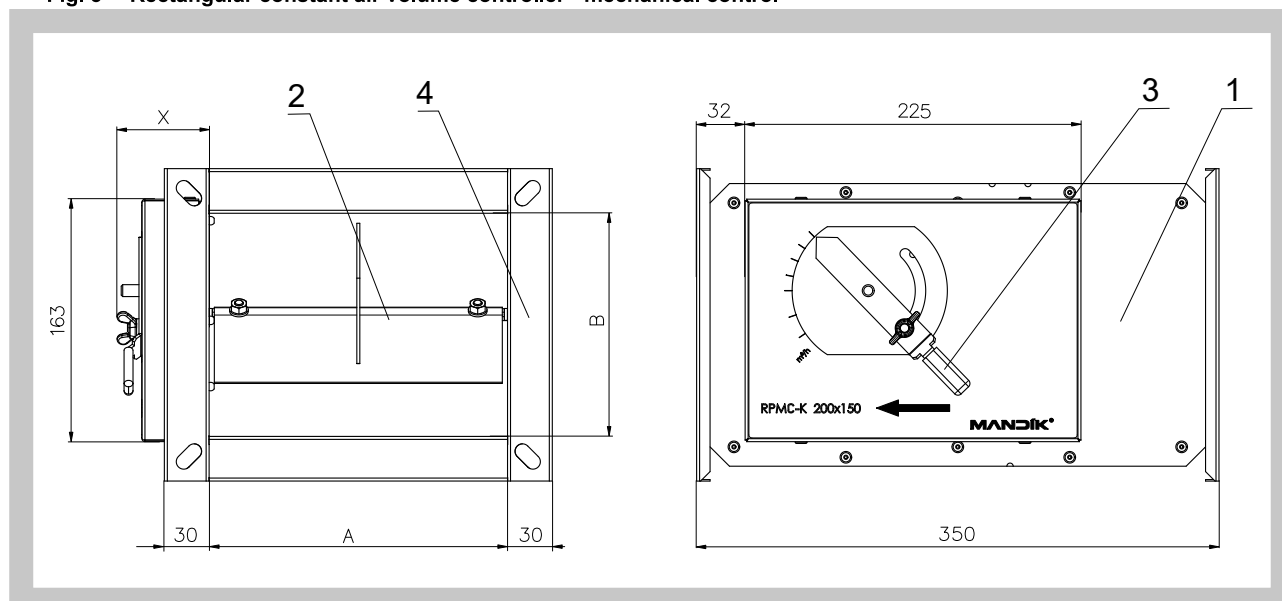
Fig. 3 Rectangular constant air volume controller - mechanical control
