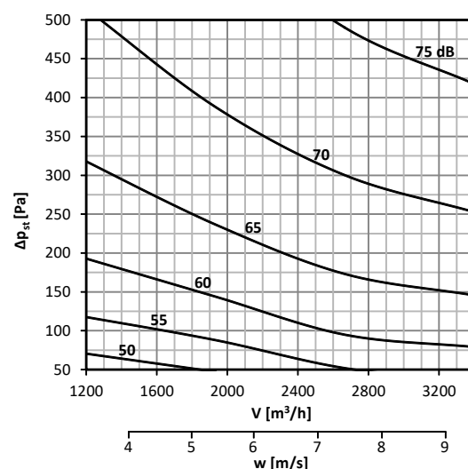
Diagram No. 12 Sound power level L_{WA} [dB(A)] inside the pipeline 400x400
