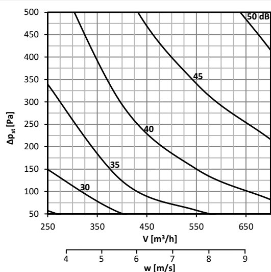
Diagram No. 49 Sound power level L_{WA} [dB(A)] radiated outside the pipeline 200x200, with insulation
