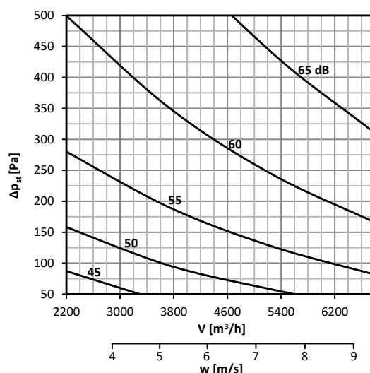
Diagram No. 41 Sound power level L_{WA} [dB(A)] radiated outside the pipeline 600x200, without insulation
