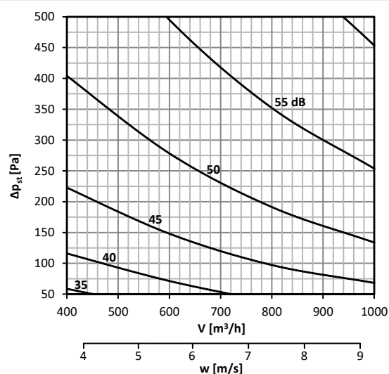
Diagram No. 27 Sound power level L_{WA} [dB(A)] radiated outside the pipeline 300x100, without insulation
