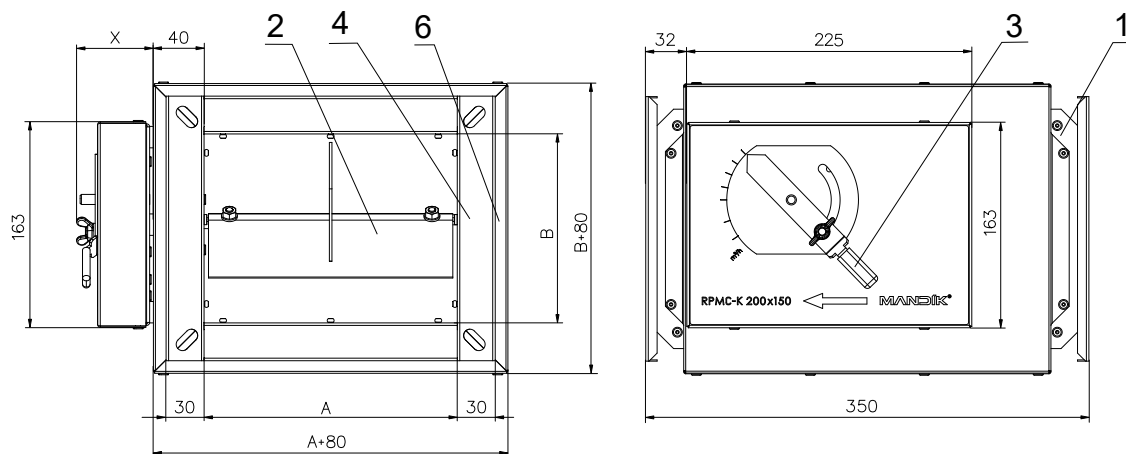
Fig. 5 Rectangular constant air volume controller - actuating mechanism
