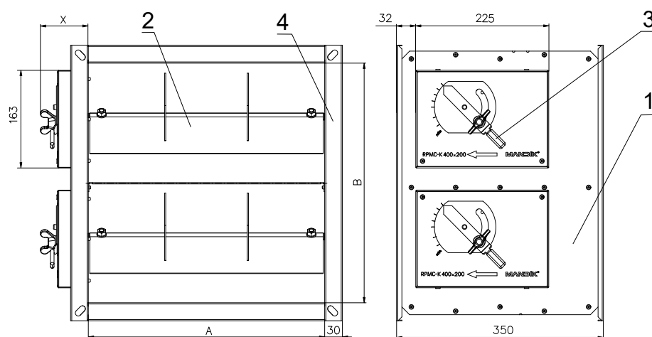
Fig. 6 Rectangular constant air volume controller - B \geq 400 mechanical control
