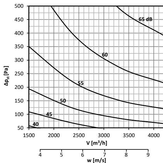
Diagram No. 34 Sound power level L_{WA} [dB(A)] radiated outside the pipeline 400x300, without insulation
