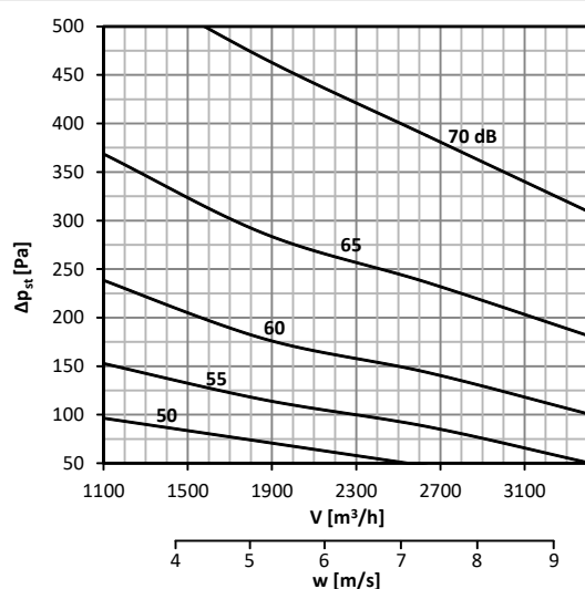
Diagram No. 15 Sound power level L_{WA} [dB(A)] inside the pipeline 500x300
