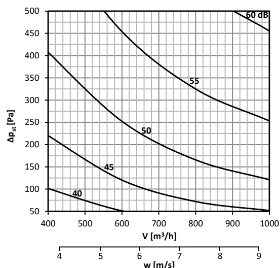
Diagram No. 29 Sound power level L_{WA} [dB(A)] radiated outside the pipeline 300x200, without insulation
