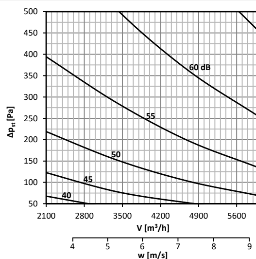
Diagram No. 45 Sound power level L_{WA} [dB(A)] radiated outside the pipeline 600x500, without insulation
