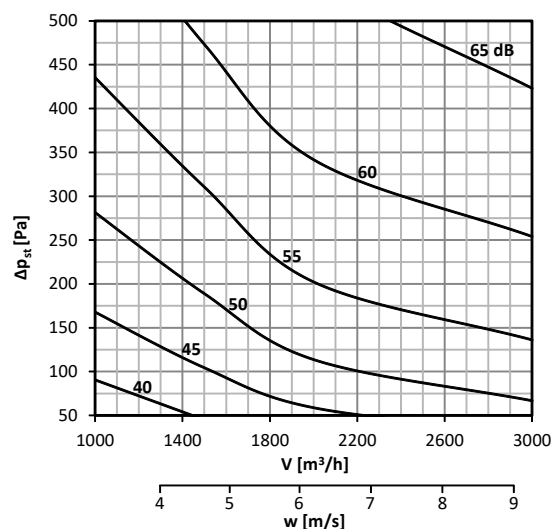
Diagram No. 33 Sound power level L_{WA} [dB(A)] radiated outside the pipeline 400x250, without insulation
