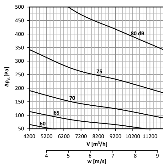
Diagram No. 23 Sound power level L_{WA} [dB(A)] inside the pipeline 600x600
