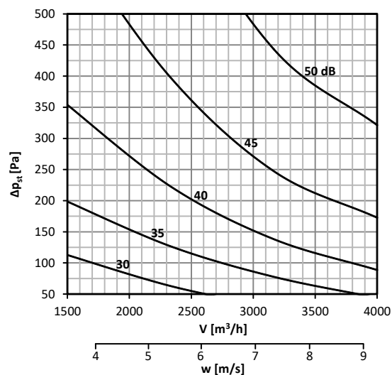
Diagram No. 64 Sound power level L_{WA} [dB(A)] radiated outside the pipeline 600x200, with insulation
