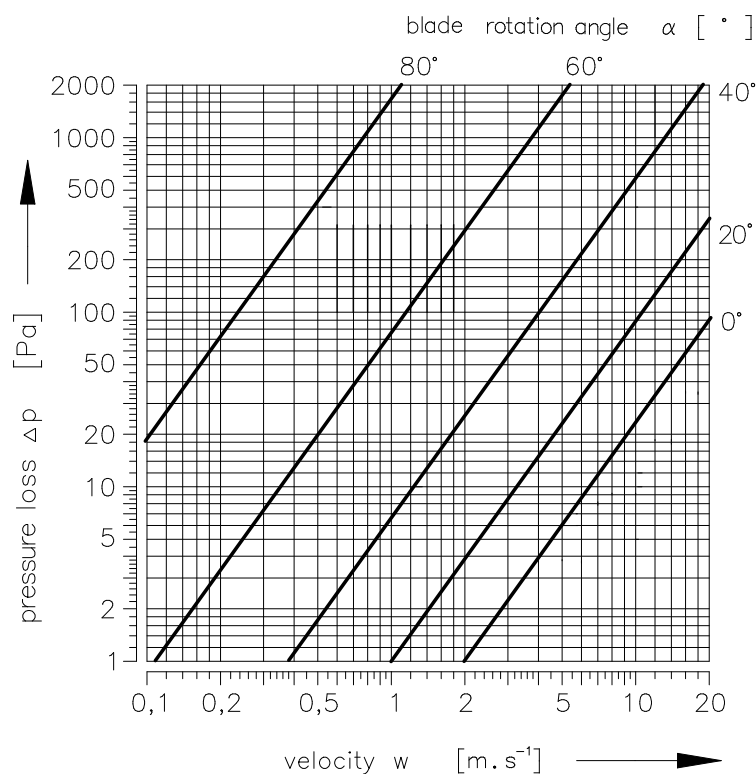
Diagram 7.1.1. Pressure losses for air density \rho = 1,2 \text{ kg.m}^{-3}
