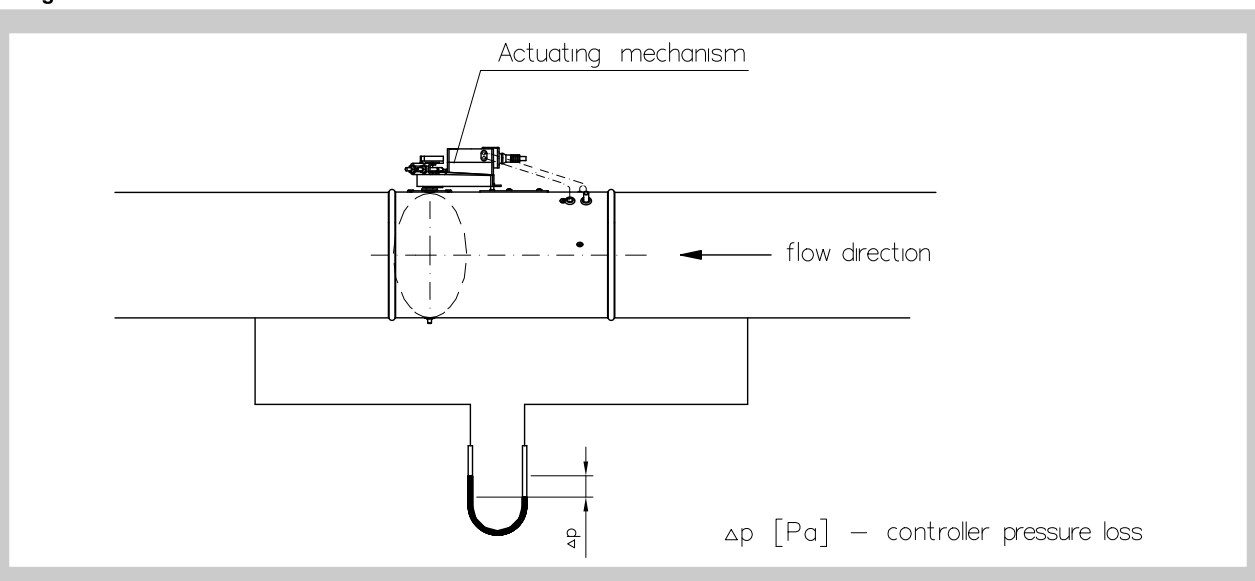
Fig. 4 Pipe pressure control
