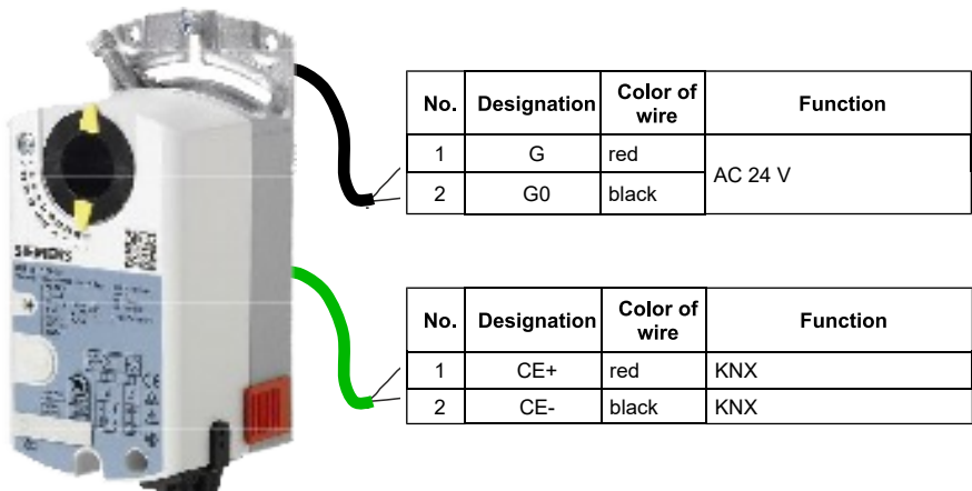
Fig. 28 GDB181.1E/KN and GLB181.1E/KN
