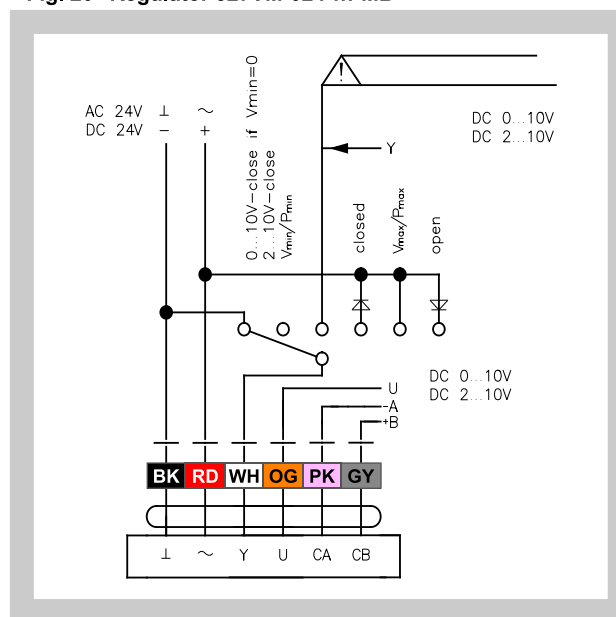
Fig. 20 Regulator 327VM-024-...-MB
