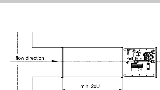
Fig. 31 Recommended distance from double branch joint
