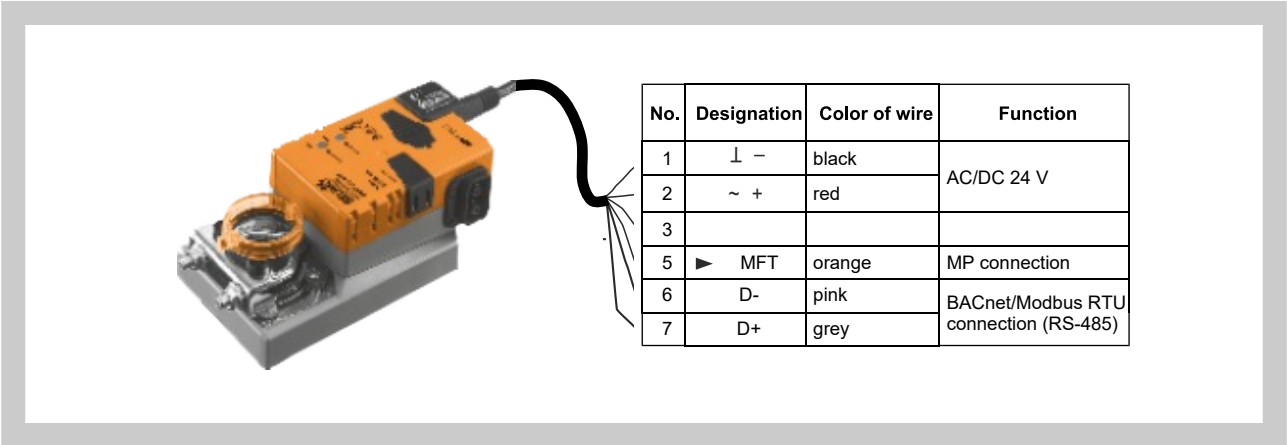
Fig. 9 Actuators LMV-D3-MOD, NMV-D3-MOD and SMV-D3-MOD
