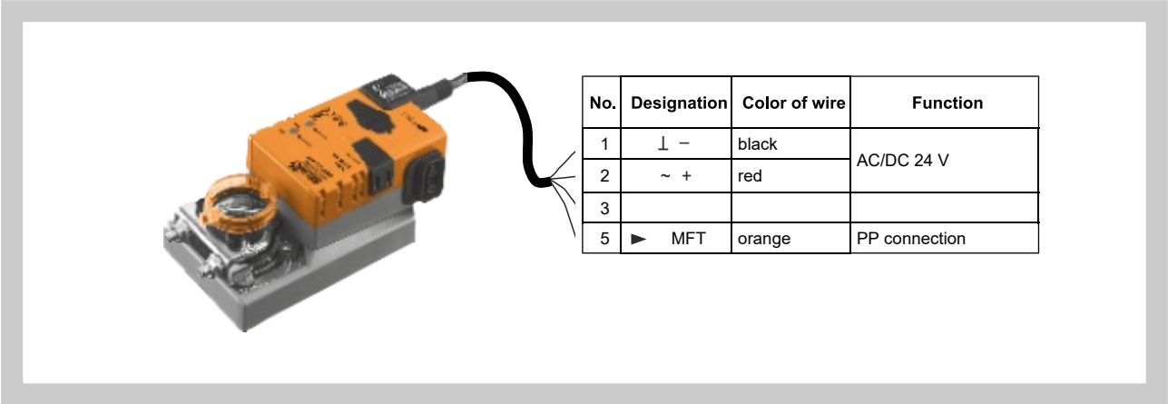
Fig. 11 Actuators LMV-D3-KNX, NMV-D3-KNX
