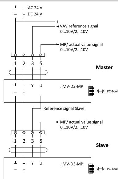
Fig. 8 Master-slave flow control with actuators LMV-D3-MP, NMV-D3-MP, SMV-D3-MP, LMV-D3-MF.1 MDK* and NMV-D3-MF.1 MDK*
