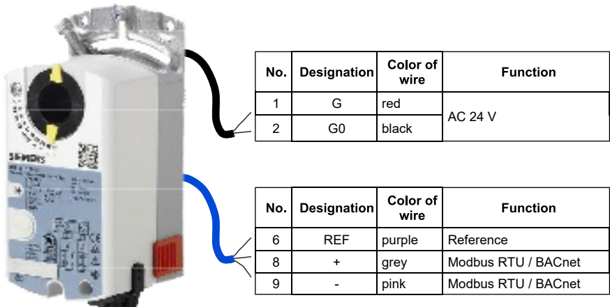
Fig. 27 GDB181.1E/BA, GLB181.1E/BA, GDB181.1E/MO and GLB181.1E/MO
