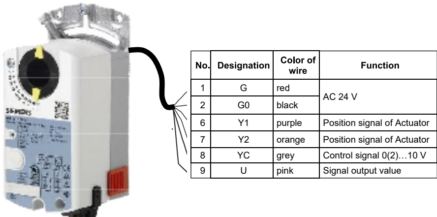
Fig. 26 GDB181.1E/3 and GLB181.1E/3
