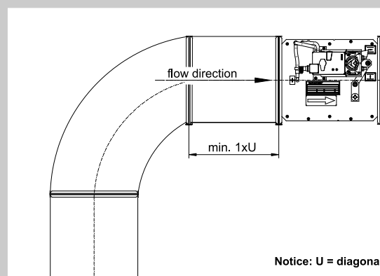
Fig. 32 Recommended distance from bend
