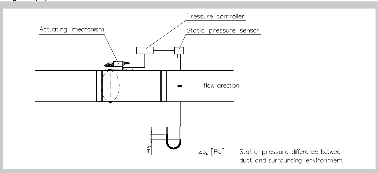
Fig. 4 Pipe pressure control
