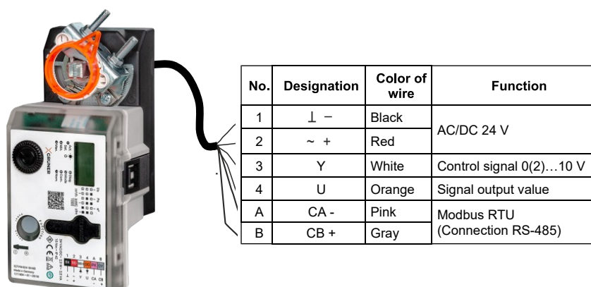
Fig. 18 Regulators 327VM-024-... -MB
