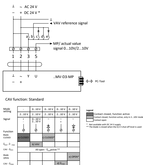
Fig. 7 Air flow control with LMV-D3-MP, NMV-D3-MP, SMV-D3-MP, LMV-D3-MF.1 MDK* and NMV-D3-MF.1 MDK*
