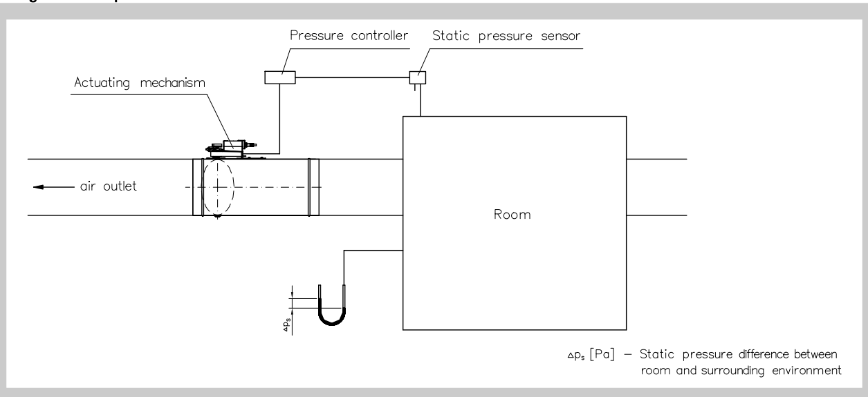
Fig. 5 Room pressure control
