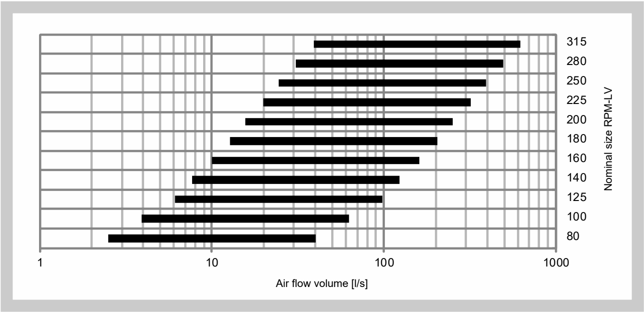
Fig. 17 Controller size selection according to air flow [l/s]
