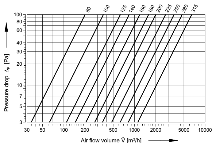
Diagram 8.1.1. Pressure drop (the values are valid when the damper of the controller is completely open)
