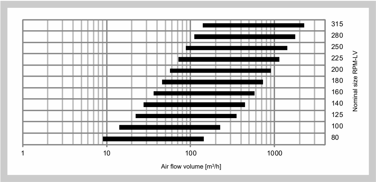
Fig. 16 Controller size selection according to air flow [m³/h]
