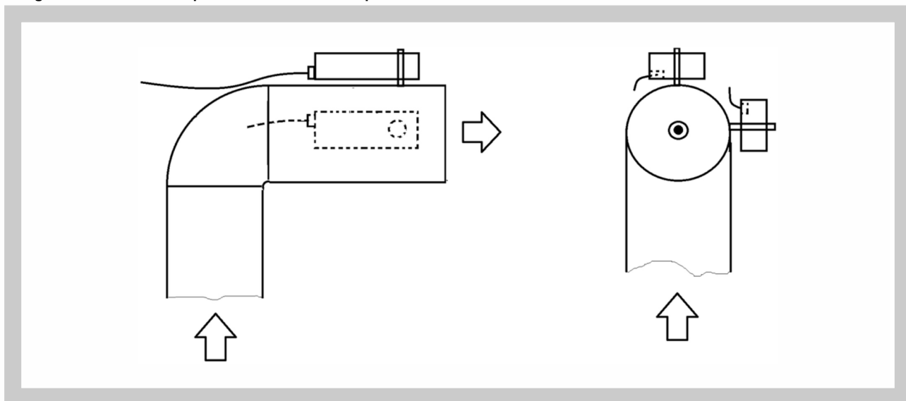
Fig. 8 Recommended positions of the elbow upstream
