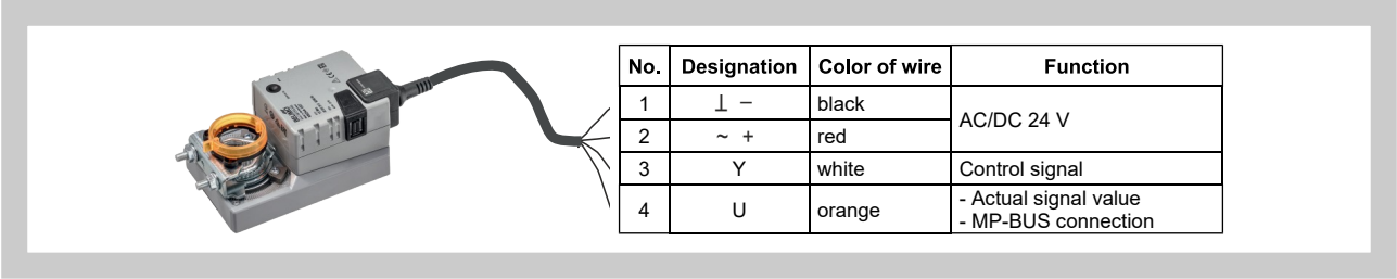
Fig. 11 Air flow control with actuator LMV-D3W-MP.1 MDK
