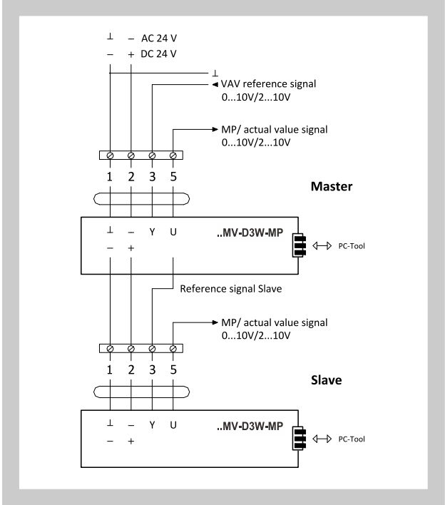
Fig. 12 Master-slave flow control with actuators LMV-D3W-MP.1 MDK
