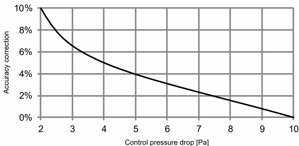
Graph 2 Accuracy of control correction for extremely small control pressure drops
